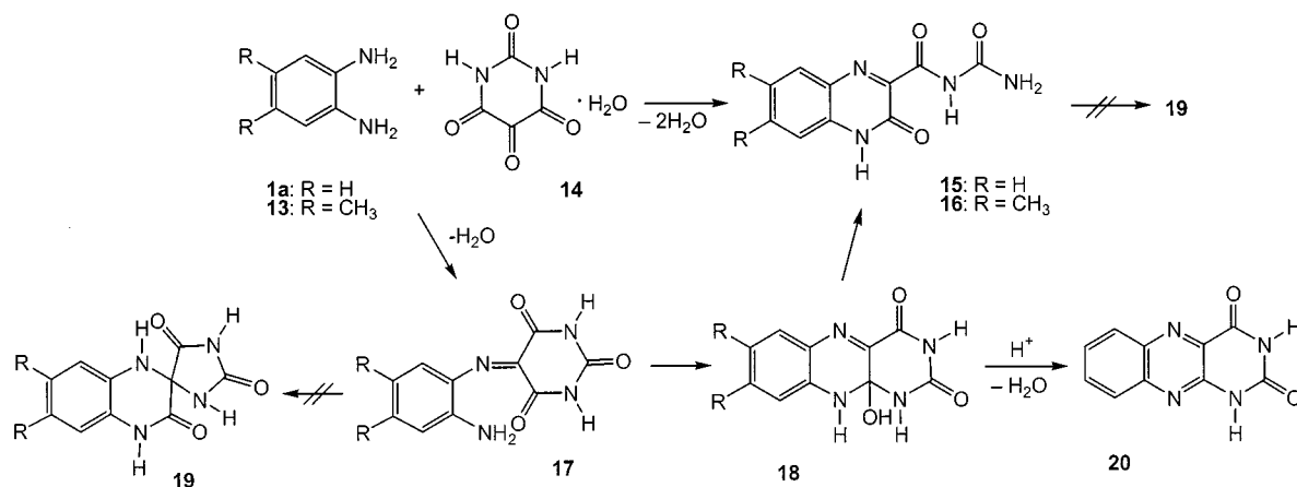
Scheme 6. The solid-state reaction between o -phenylenediamines 1a/13 and alloxane hydrate ( 14 ) to give 15/16 (and in the presence of acid also 20 )
