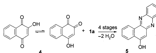
Scheme 2. Quantitative synthesis of benzo[a]phenazin-5-ol ( 5 )
