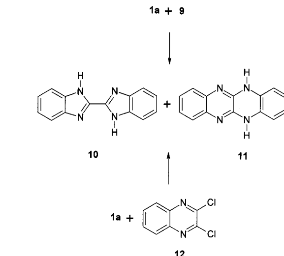
Scheme 5. Solvent-free syntheses of mixtures of the compounds 10 and fluoflavin ( 11 )
