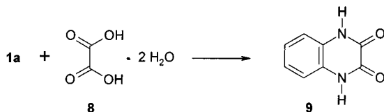
Scheme 4. Quantitative condensation between o -phenylenediamine and oxalic acid
