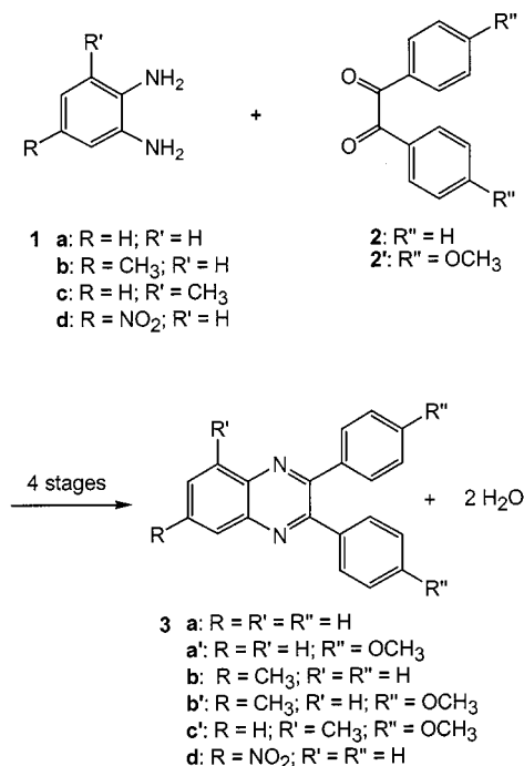
Scheme 1. Quantitative synthesis of quinoxaline derivatives
