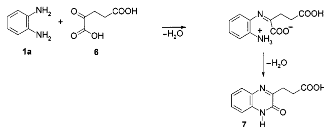
Scheme 3. Quantitative condensation between o -phenylenediamine and 2-oxoglutaric acid
